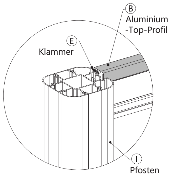
Detail 2.8-1
